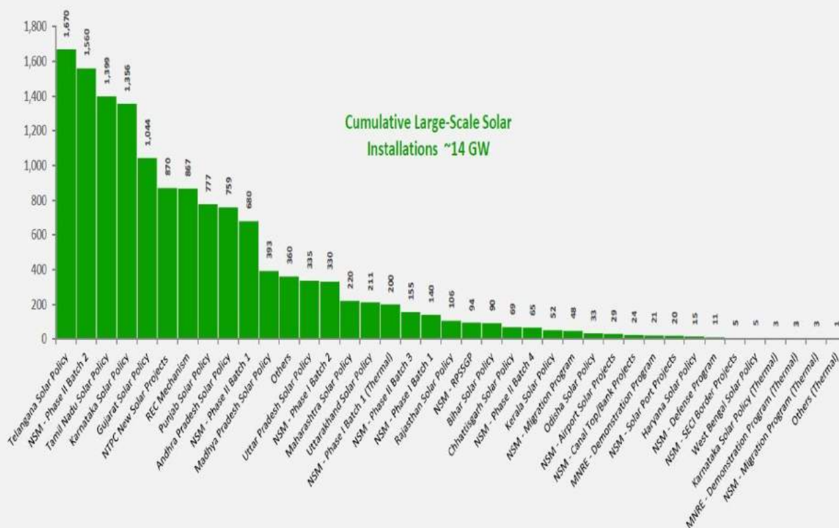
All India Cumulative Utility-Scale Solar Installations By Policy Type (MW)
